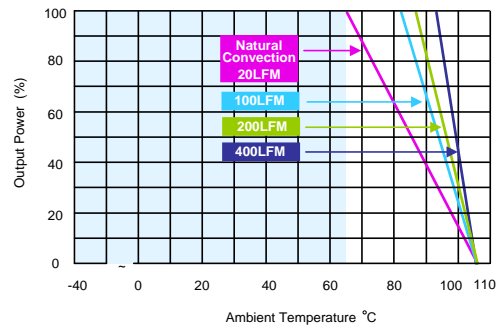
MJW25-24S033, MJW25-48S033 Derating Curve with Heatsink
